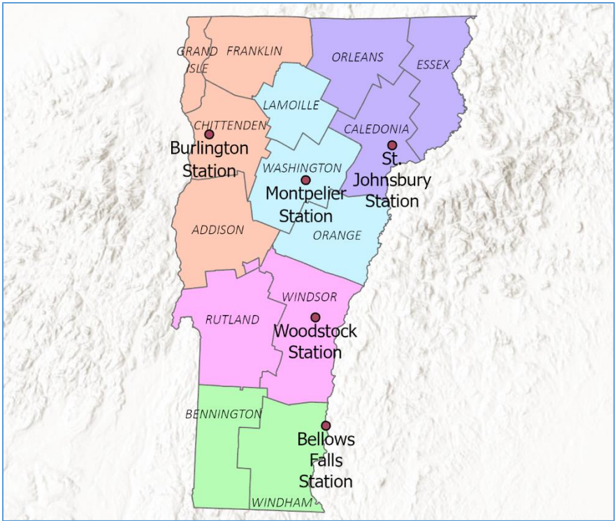
Figure 2. Distribution of five climate stations utilized in the WEPP:Road model.
