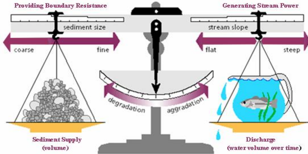
Figure 11. Lane's balance of sediment supply and sediment size with slope and discharge (Lane, 1955).
