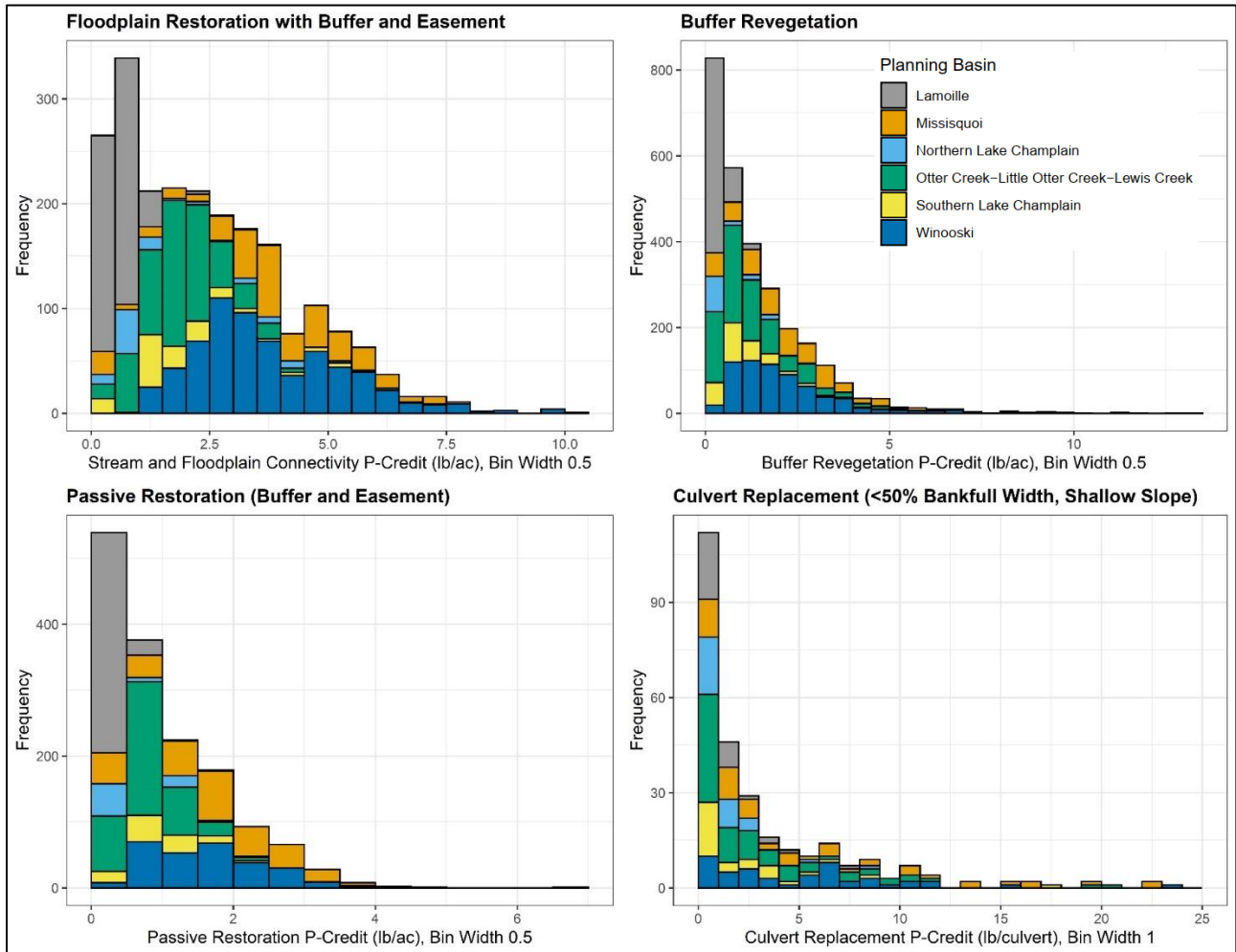
Figure 18. Sample histograms of P-credits for simulated stream and floodplain connectivity projects.
