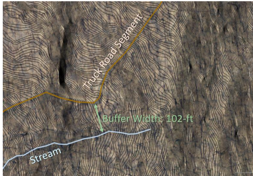
Figure 16. Buffer width example.
