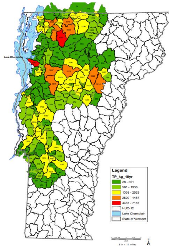
Figure 6. Lake Champlain sub-basin phosphorus load allocations.
