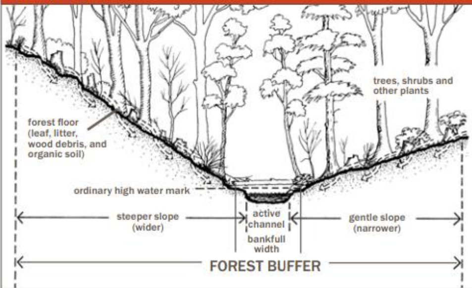
Figure 17. Vermont AMP Forest Buffer Specifications.
